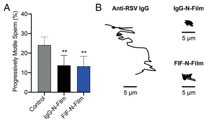
Fig. 4. FIF-N-Film maintains the trapping potency of IgG-N-Film. (A) The trapping potency of the indicated Abs (25 \mu\text{g/mL} ) measured by quantifying fluorescently labeled PM sperm in Ab-treated CVM using neural network tracker analysis software. Purified sperm at the final concentration of 5.8 \times 10^4 PM sperm/mL was used. Data were obtained from n = 6 independent experiments using 6 unique combinations of semen and CVM specimens. P values were calculated using a one-tailed t test. ** P < 0.01 . Data represent mean \pm SD. (B) Representative 4-s traces of sperm within one SE mean of average path velocity at a timescale \tau of 1 s in CVM treated with control (anti-RSV IgG), IgG-N-Film, and FIF-N-Film.
